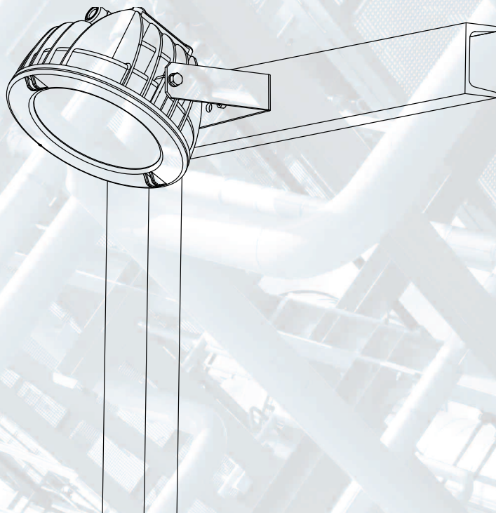
Example of wall or structure mounting
