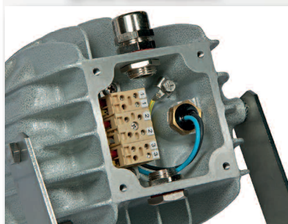
Ex e terminal housing for a quick connection
