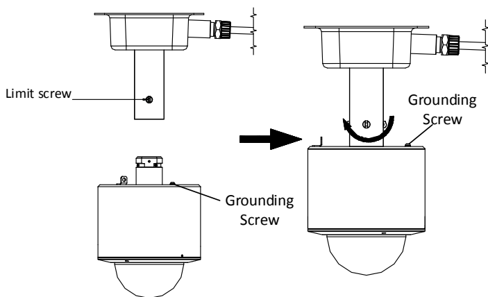
Figure 2-9 Fix the Device to the Bracket
