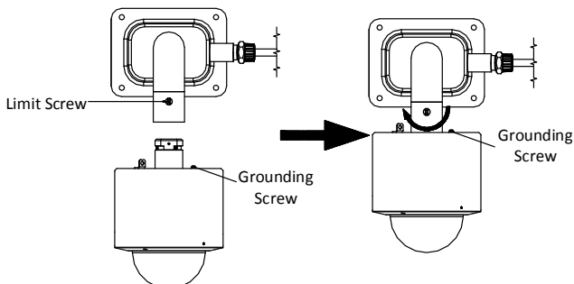
Figure 2-5 Fix the Device to the Bracket
