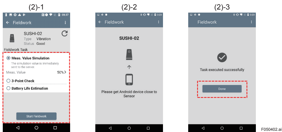
Figure 5-14 Execute Fieldwork
