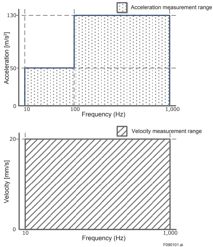
Figure 9-1 Measurable Range
