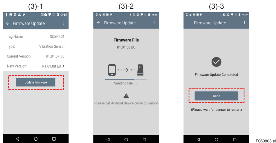
Figure 6-11 Firmware Update
